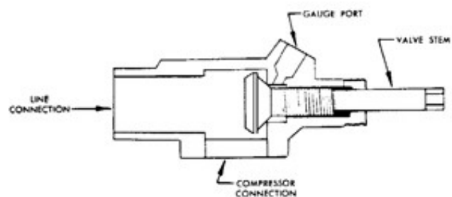
Valve Backseated
