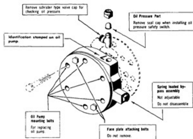
TYPICAL Copeland OIL PUMP
