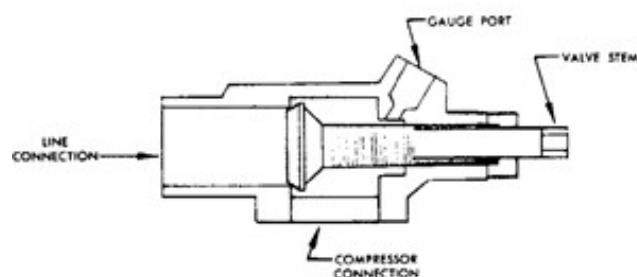
Valve Frontseated
